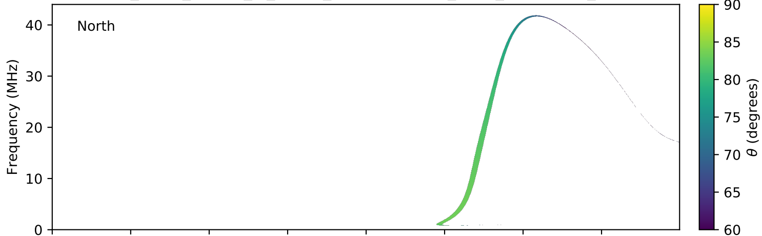
expres_earth_jupiter_io_jrm09_lossc-wid1deg_3kev_20171229_v01.cdf
