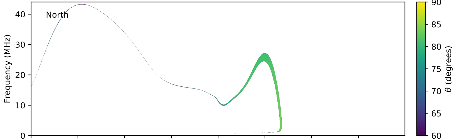
expres_earth_jupiter_io_jrm09_lossc-wid1deg_3kev_20171228_v01.cdf
