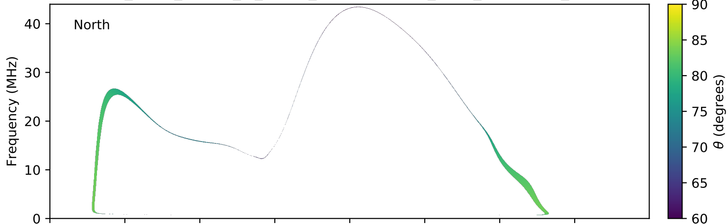
expres_earth_jupiter_io_jrm09_lossc-wid1deg_3kev_20171226_v01.cdf
