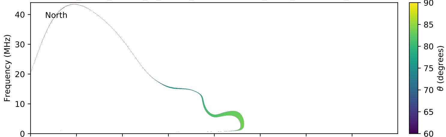
expres_earth_jupiter_io_jrm09_lossc-wid1deg_3kev_20171221_v01.cdf
