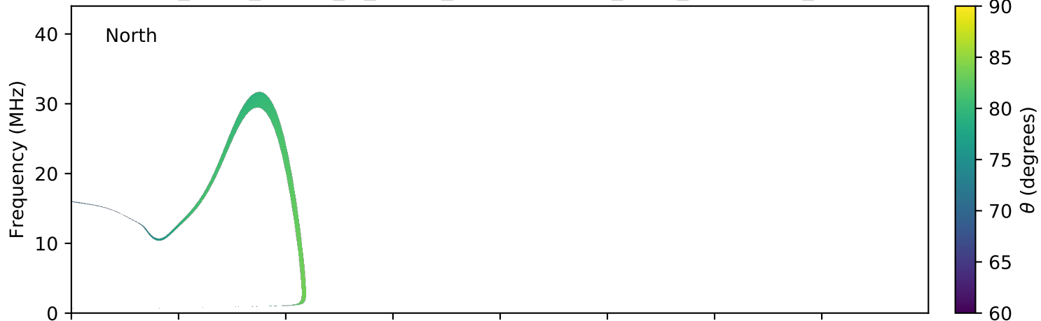
expres_earth_jupiter_io_jrm09_lossc-wid1deg_3kev_20171216_v01.cdf
