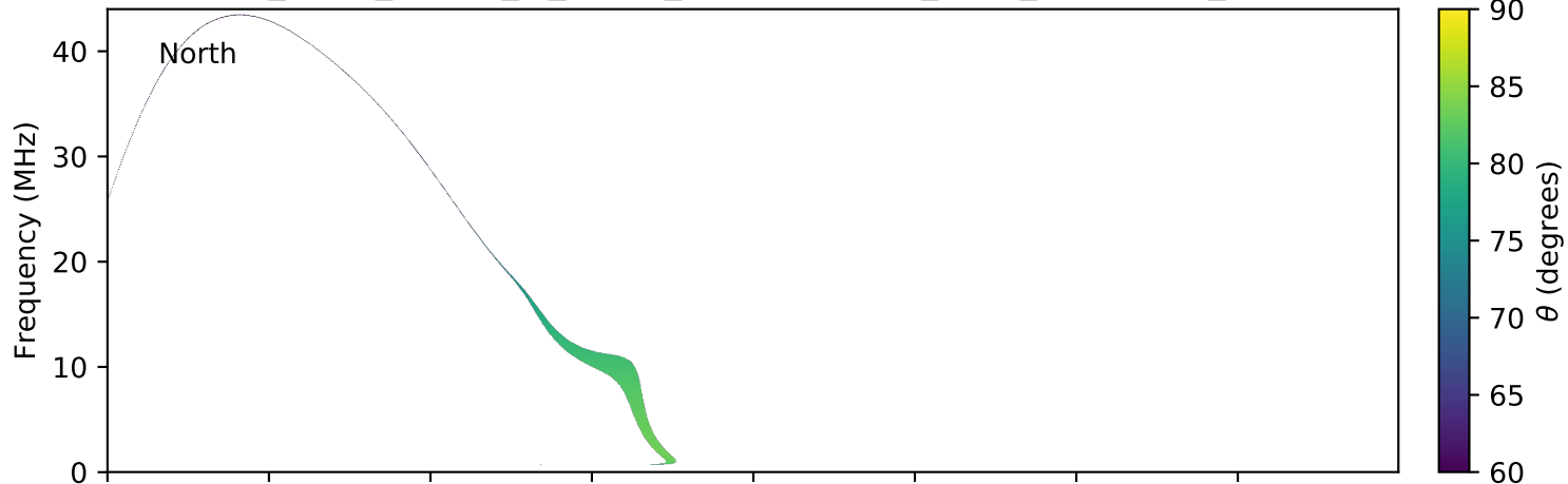
expres_earth_jupiter_io_jrm09_lossc-wid1deg_3kev_20171214_v01.cdf
