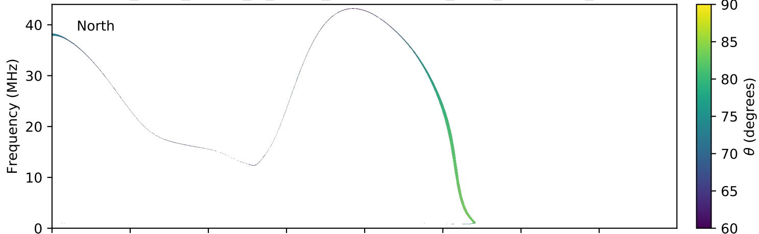
expres_earth_jupiter_io_jrm09_lossc-wid1deg_3kev_20171212_v01.cdf
