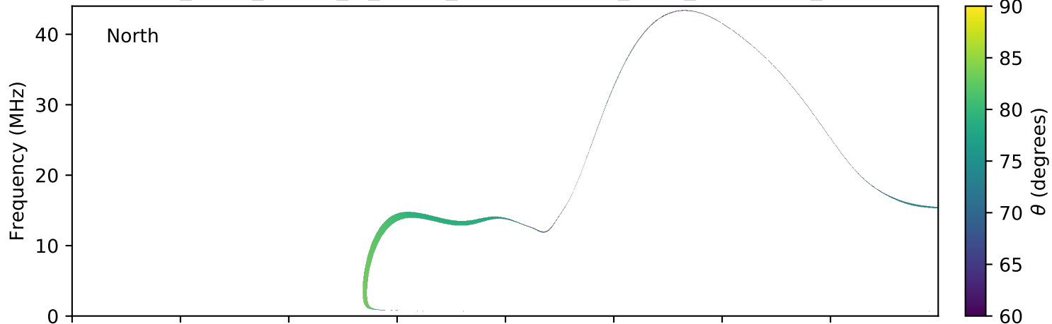
expres_earth_jupiter_io_jrm09_lossc-wid1deg_3kev_20171208_v01.cdf
