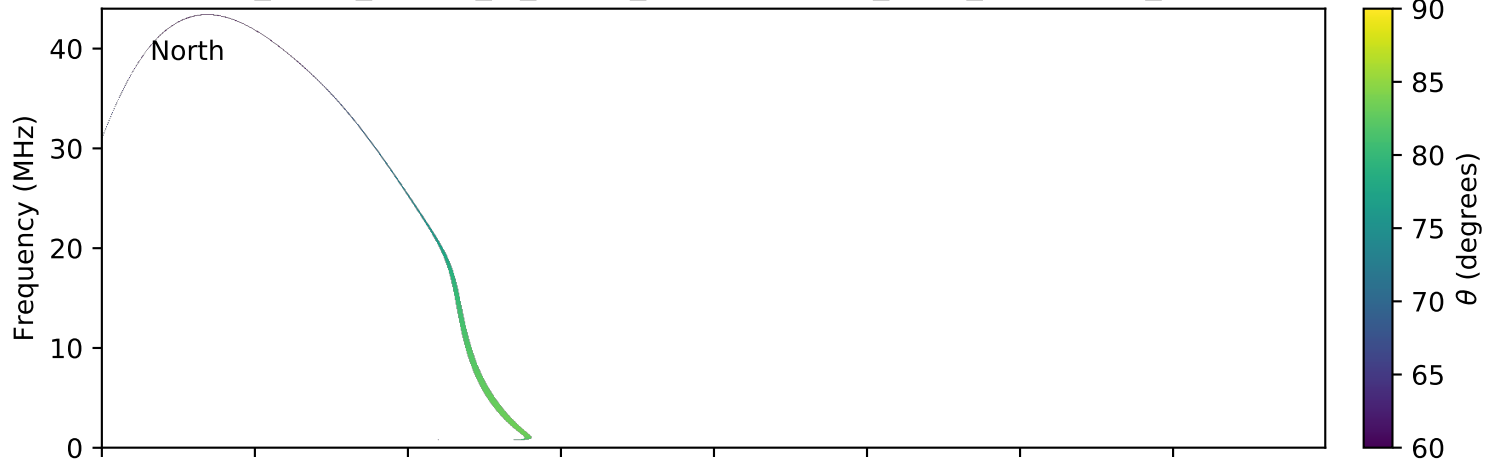
expres_earth_jupiter_io_jrm09_lossc-wid1deg_3kev_20171207_v01.cdf
