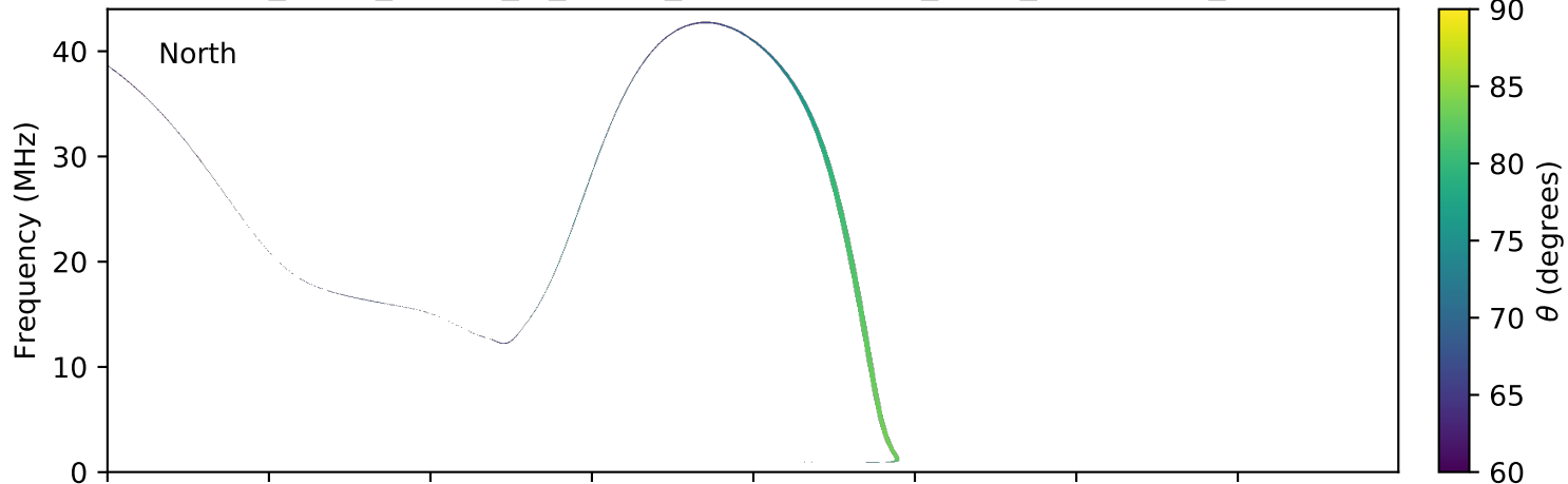
expres_earth_jupiter_io_jrm09_lossc-wid1deg_3kev_20171205_v01.cdf
