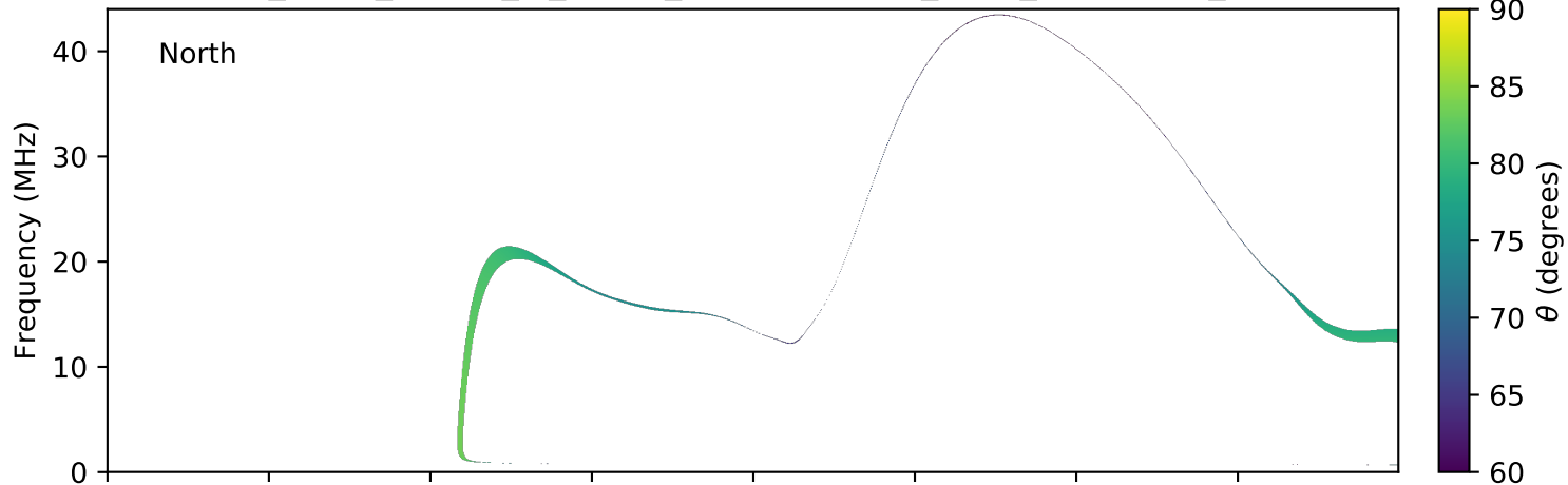
expres_earth_jupiter_io_jrm09_lossc-wid1deg_3kev_20171201_v01.cdf
