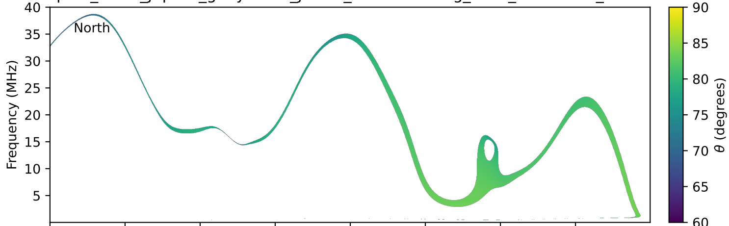
expres_earth_jupiter_ganymede_jrm33_lossc-wid1deg_3kev_20171205_v11.cdf
