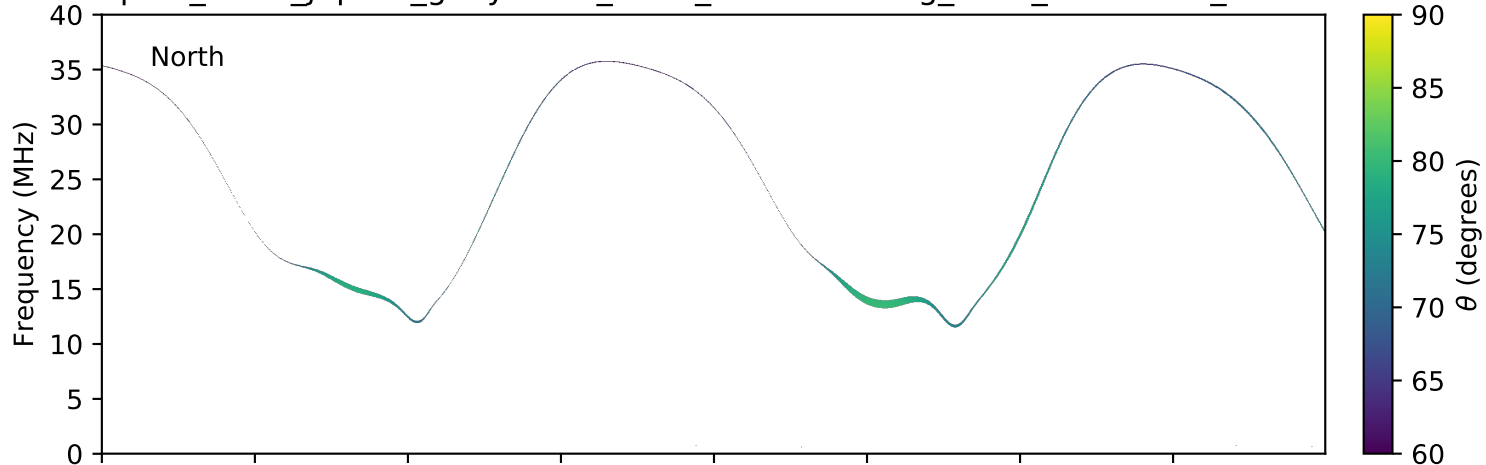
expres_earth_jupiter_ganymede_isaac_lossc-wid1deg_3kev_20171229_v01.cdf
