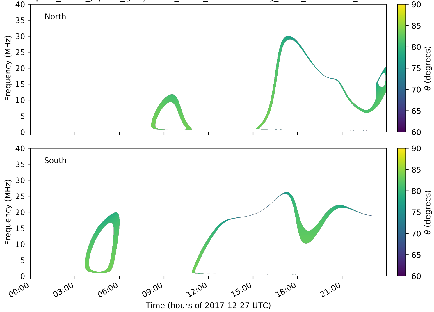
expres_earth_jupiter_ganymede_isaac_lossc-wid1deg_3kev_20171227_v01.cdf
