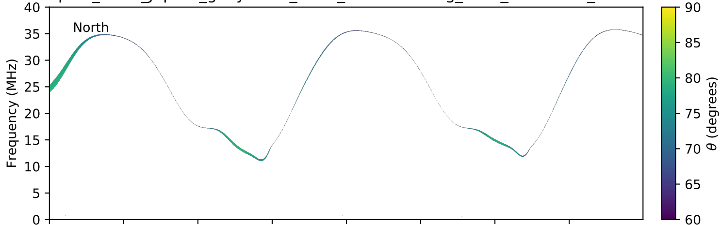
expres_earth_jupiter_ganymede_isaac_lossc-wid1deg_3kev_20171221_v01.cdf
