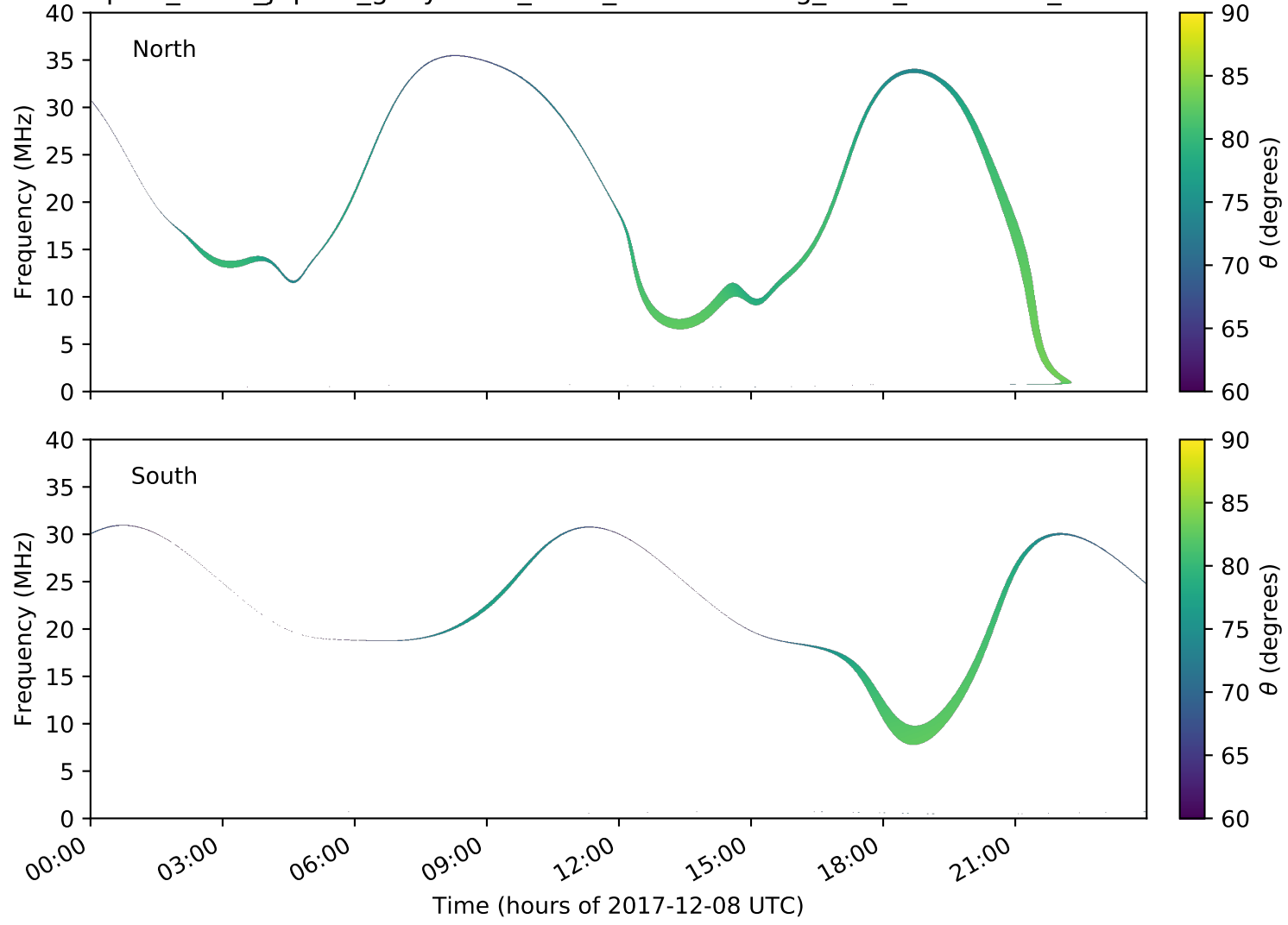
expres_earth_jupiter_ganymede_isaac_lossc-wid1deg_3kev_20171208_v01.cdf
