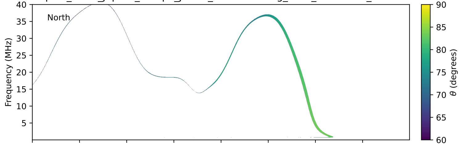
expres_earth_jupiter_europa_jrm33_lossc-wid1deg_3kev_20171221_v11.cdf
