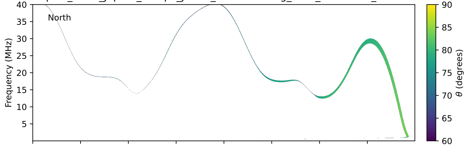
expres_earth_jupiter_europa_jrm33_lossc-wid1deg_3kev_20171217_v11.cdf
