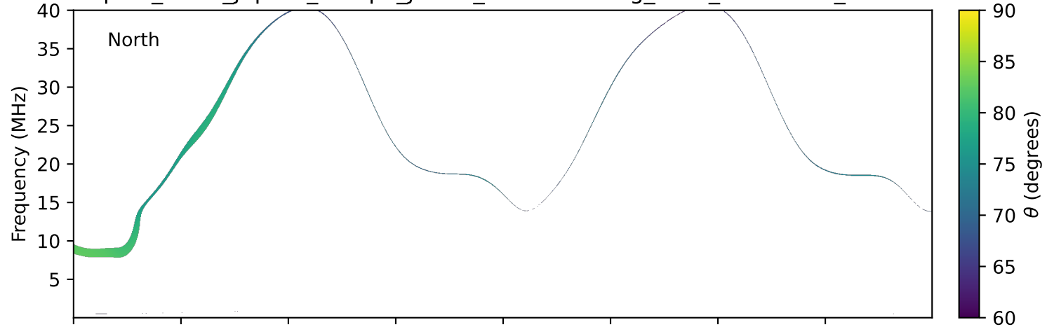
expres_earth_jupiter_europa_jrm33_lossc-wid1deg_3kev_20171213_v11.cdf
