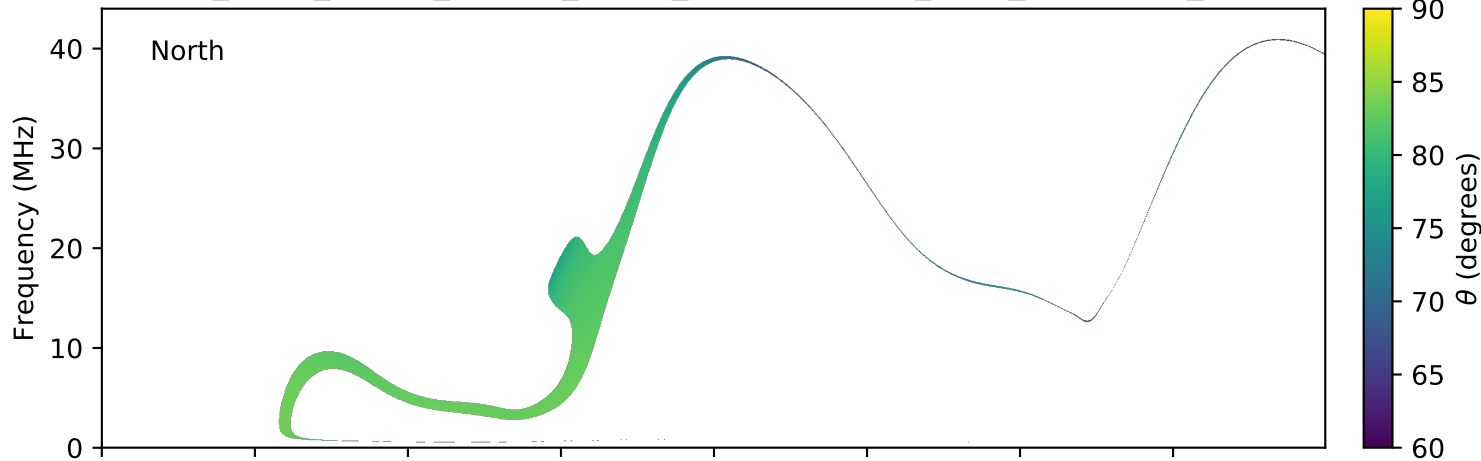
expres_earth_jupiter_europa_jrm09_lossc-wid1deg_3kev_20171221_v01.cdf
