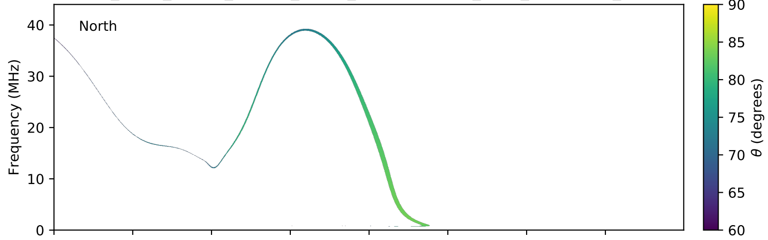
expres_earth_jupiter_europa_jrm09_lossc-wid1deg_3kev_20171215_v01.cdf
