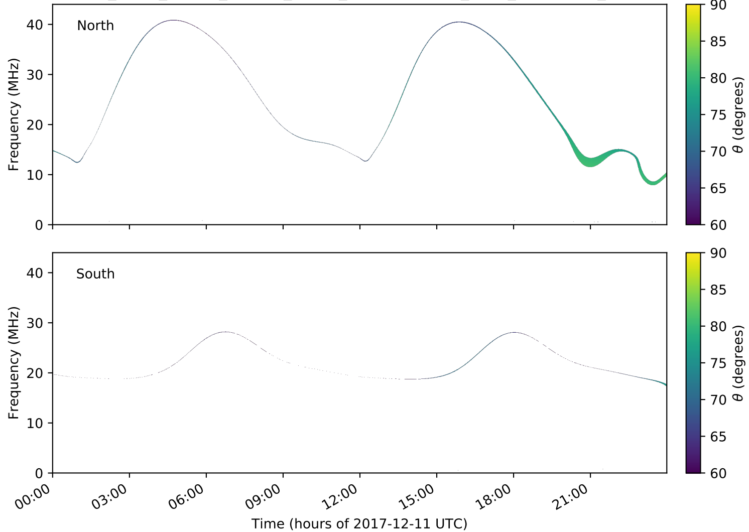
expres_earth_jupiter_europa_jrm09_lossc-wid1deg_3kev_20171211_v01.cdf
