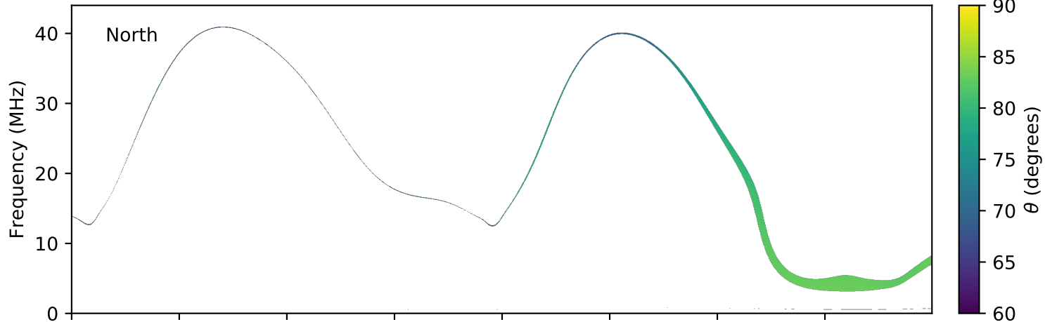
expres_earth_jupiter_europa_jrm09_lossc-wid1deg_3kev_20171204_v01.cdf
