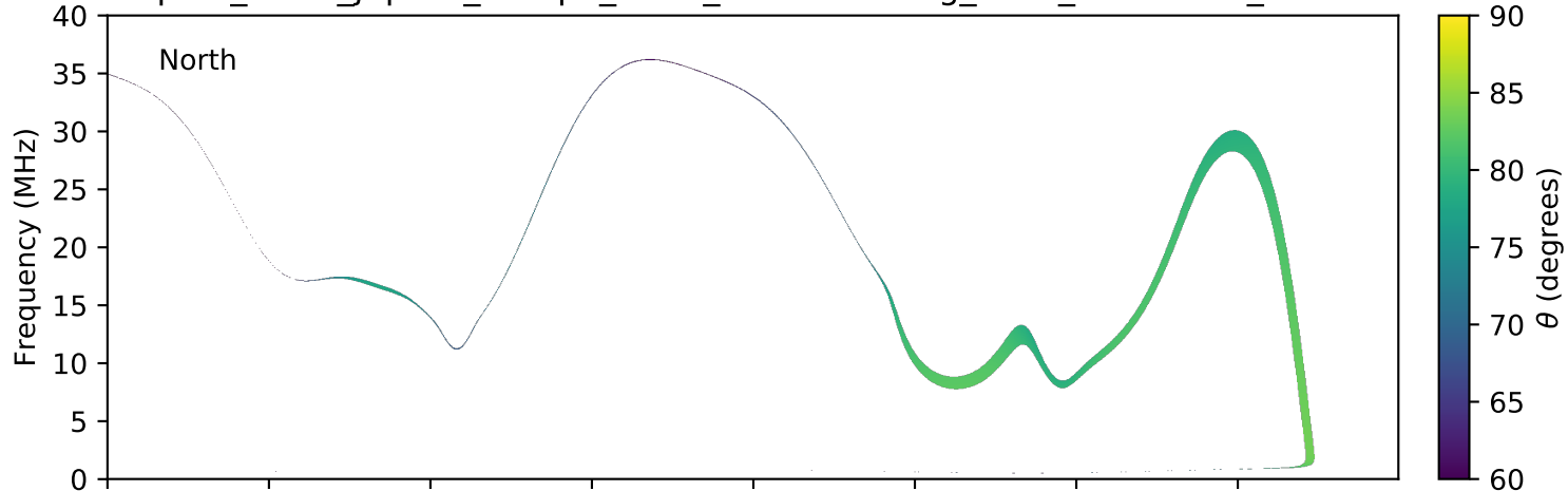
expres_earth_jupiter_europa_isaac_lossc-wid1deg_3kev_20171229_v01.cdf
