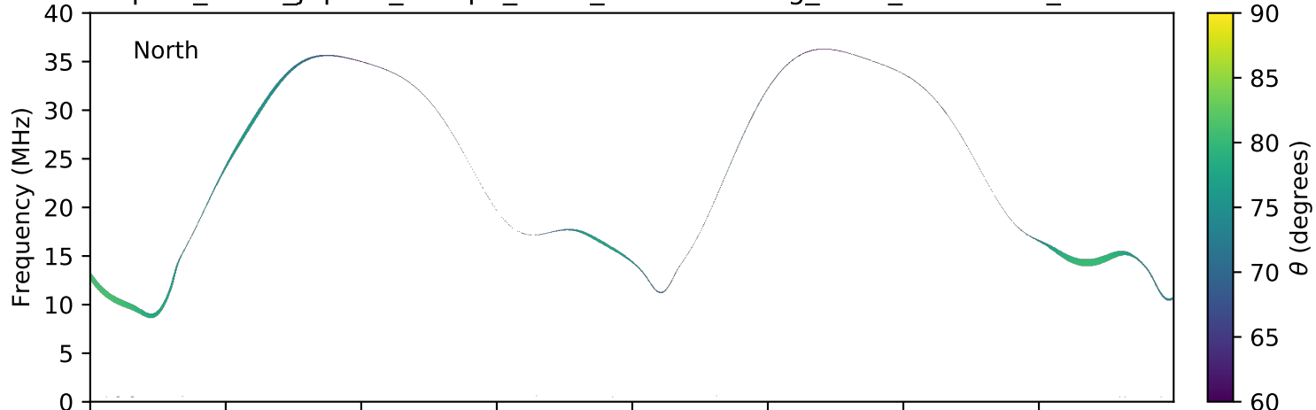
expres_earth_jupiter_europa_isaac_lossc-wid1deg_3kev_20171225_v01.cdf
