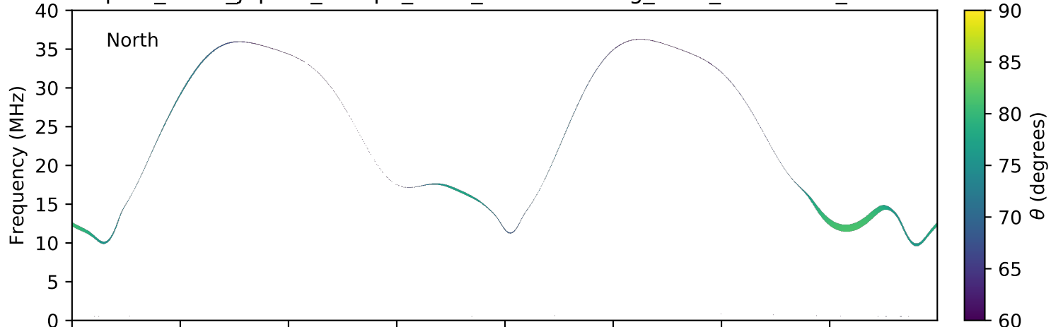
expres_earth_jupiter_europa_isaac_lossc-wid1deg_3kev_20171218_v01.cdf
