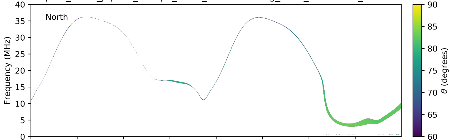
expres_earth_jupiter_europa_isaac_lossc-wid1deg_3kev_20171204_v01.cdf
