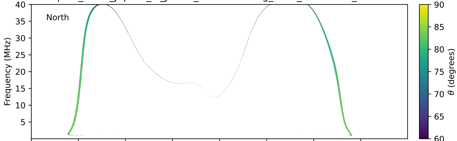
expres_earth_jupiter_io_jrm33_lossc-wid1deg_3kev_20171129_v11.cdf
