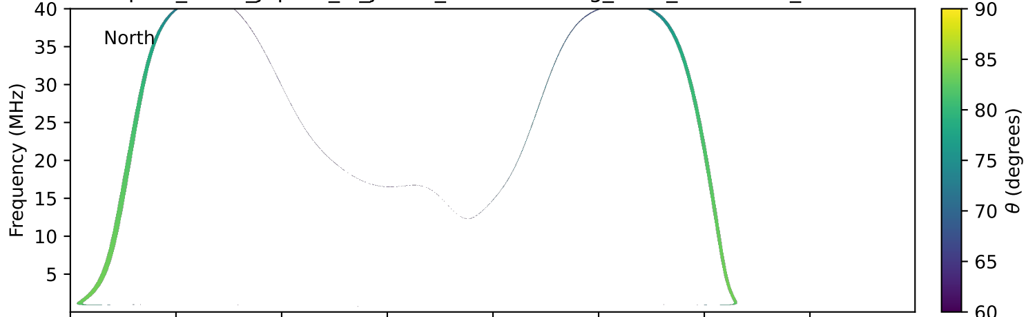
expres_earth_jupiter_io_jrm33_lossc-wid1deg_3kev_20171122_v11.cdf
