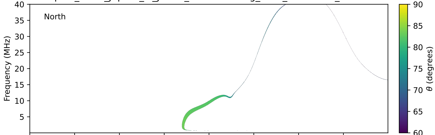
expres_earth_jupiter_io_jrm33_lossc-wid1deg_3kev_20171109_v11.cdf
