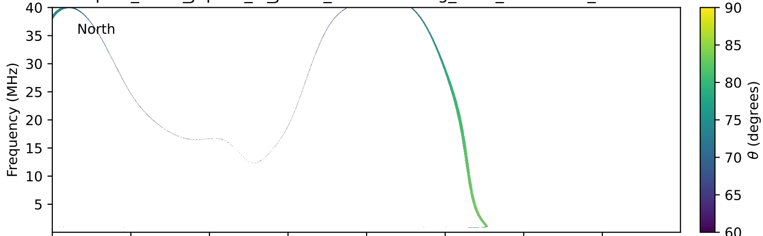
expres_earth_jupiter_io_jrm33_lossc-wid1deg_3kev_20171106_v11.cdf
