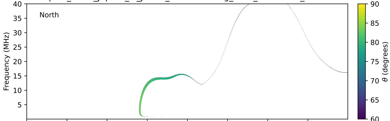
expres_earth_jupiter_io_jrm33_lossc-wid1deg_3kev_20171102_v11.cdf
