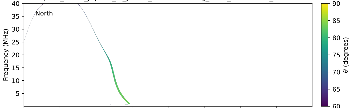
expres_earth_jupiter_io_jrm33_lossc-wid1deg_3kev_20171101_v11.cdf
