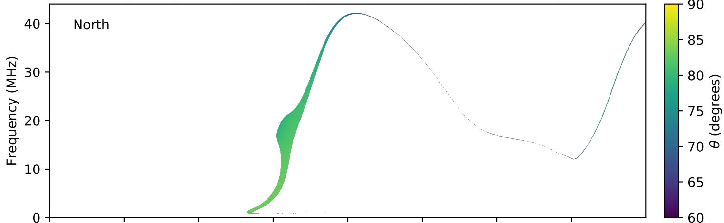
expres_earth_jupiter_io_jrm09_lossc-wid1deg_3kev_20171115_v01.cdf
