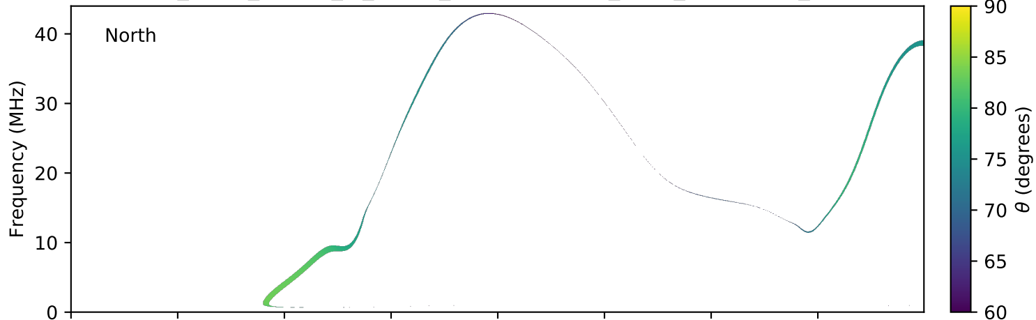
expres_earth_jupiter_io_jrm09_lossc-wid1deg_3kev_20171108_v01.cdf
