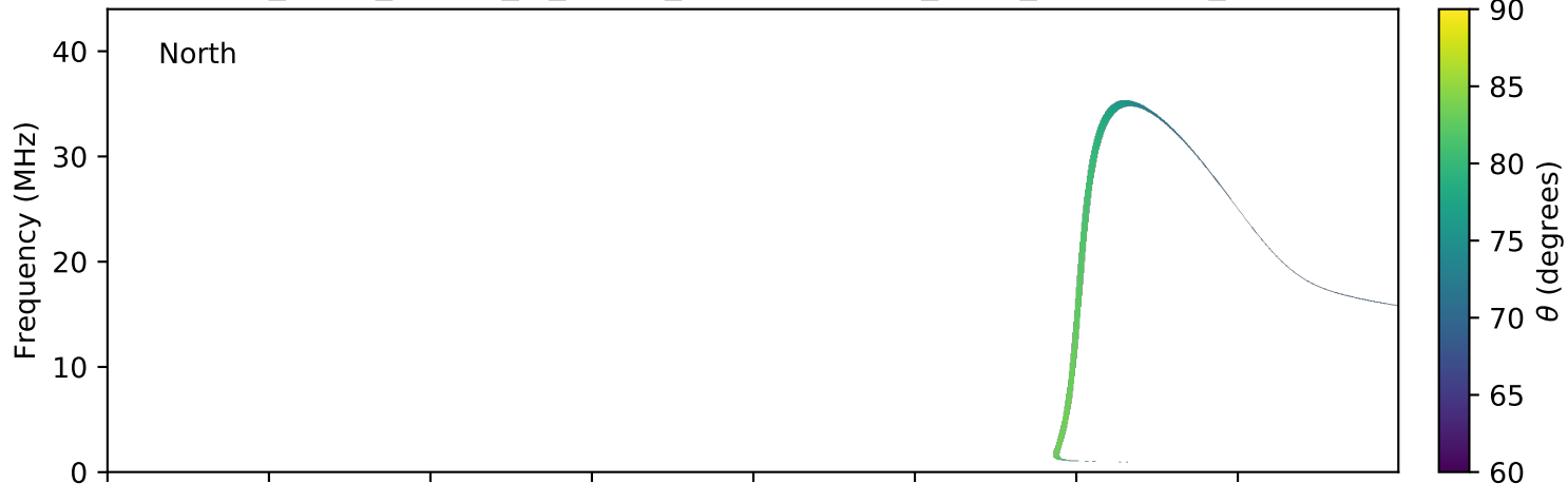
expres_earth_jupiter_io_jrm09_lossc-wid1deg_3kev_20171104_v01.cdf
