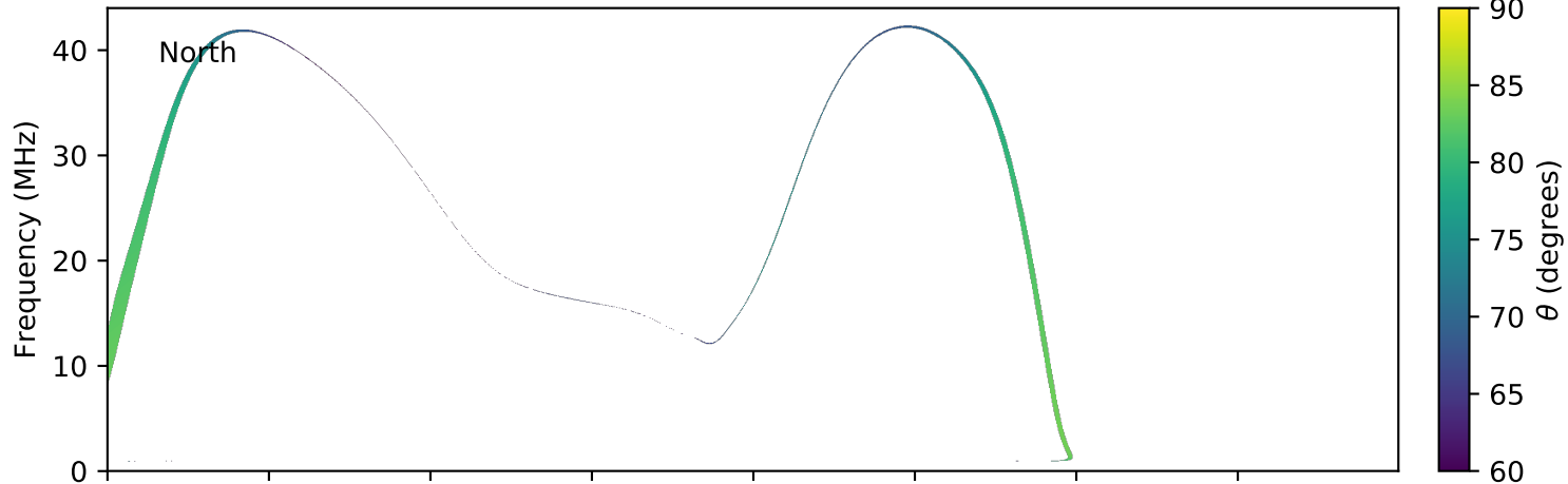
expres_earth_jupiter_io_jrm09_lossc-wid1deg_3kev_20171103_v01.cdf
