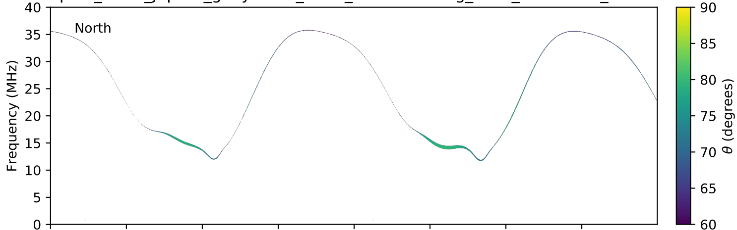
expres_earth_jupiter_ganymede_isaac_lossc-wid1deg_3kev_20171123_v01.cdf
