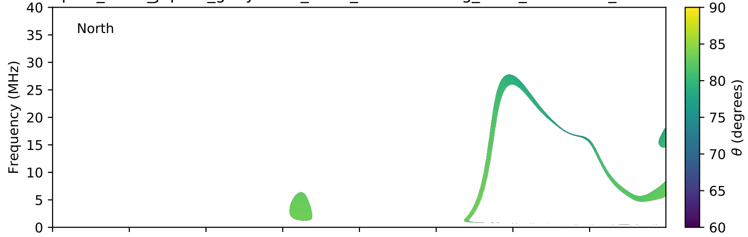
expres_earth_jupiter_ganymede_isaac_lossc-wid1deg_3kev_20171121_v01.cdf
