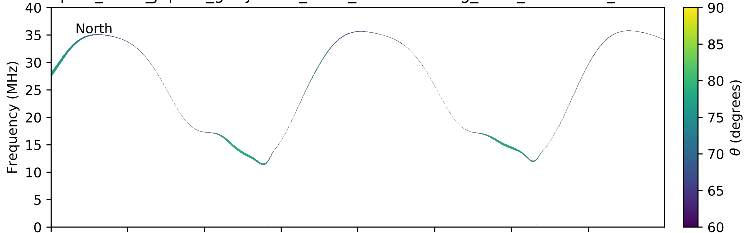
expres_earth_jupiter_ganymede_isaac_lossc-wid1deg_3kev_20171108_v01.cdf
