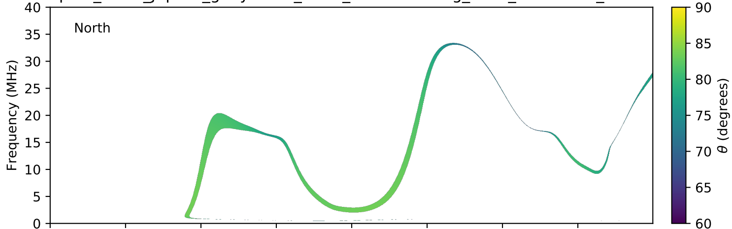
expres_earth_jupiter_ganymede_isaac_lossc-wid1deg_3kev_20171107_v01.cdf
