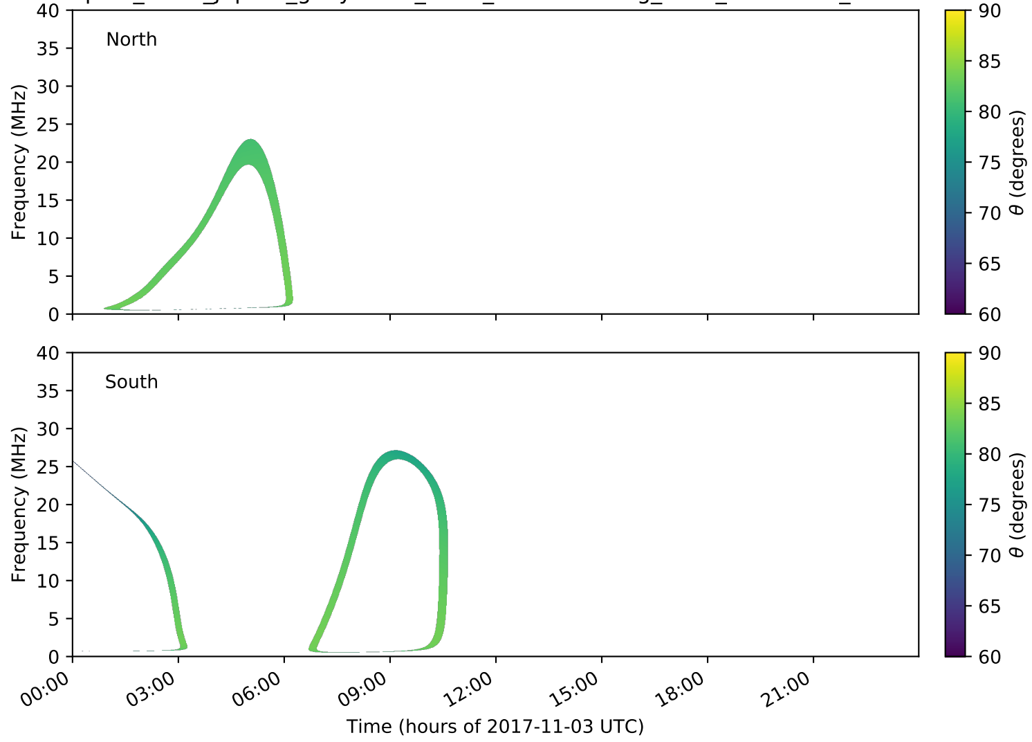
expres_earth_jupiter_ganymede_isaac_lossc-wid1deg_3kev_20171103_v01.cdf
