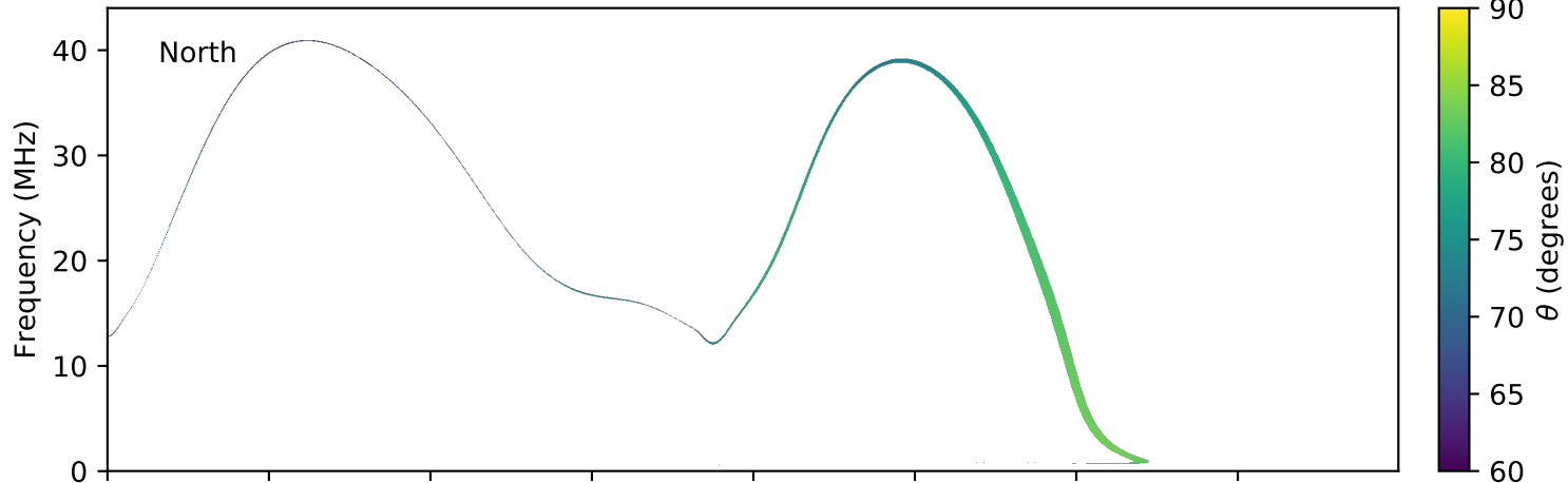
expres_earth_jupiter_europa_jrm09_lossc-wid1deg_3kev_20171127_v01.cdf
