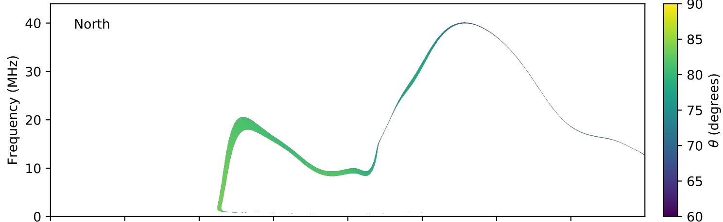
expres_earth_jupiter_europa_jrm09_lossc-wid1deg_3kev_20171126_v01.cdf
