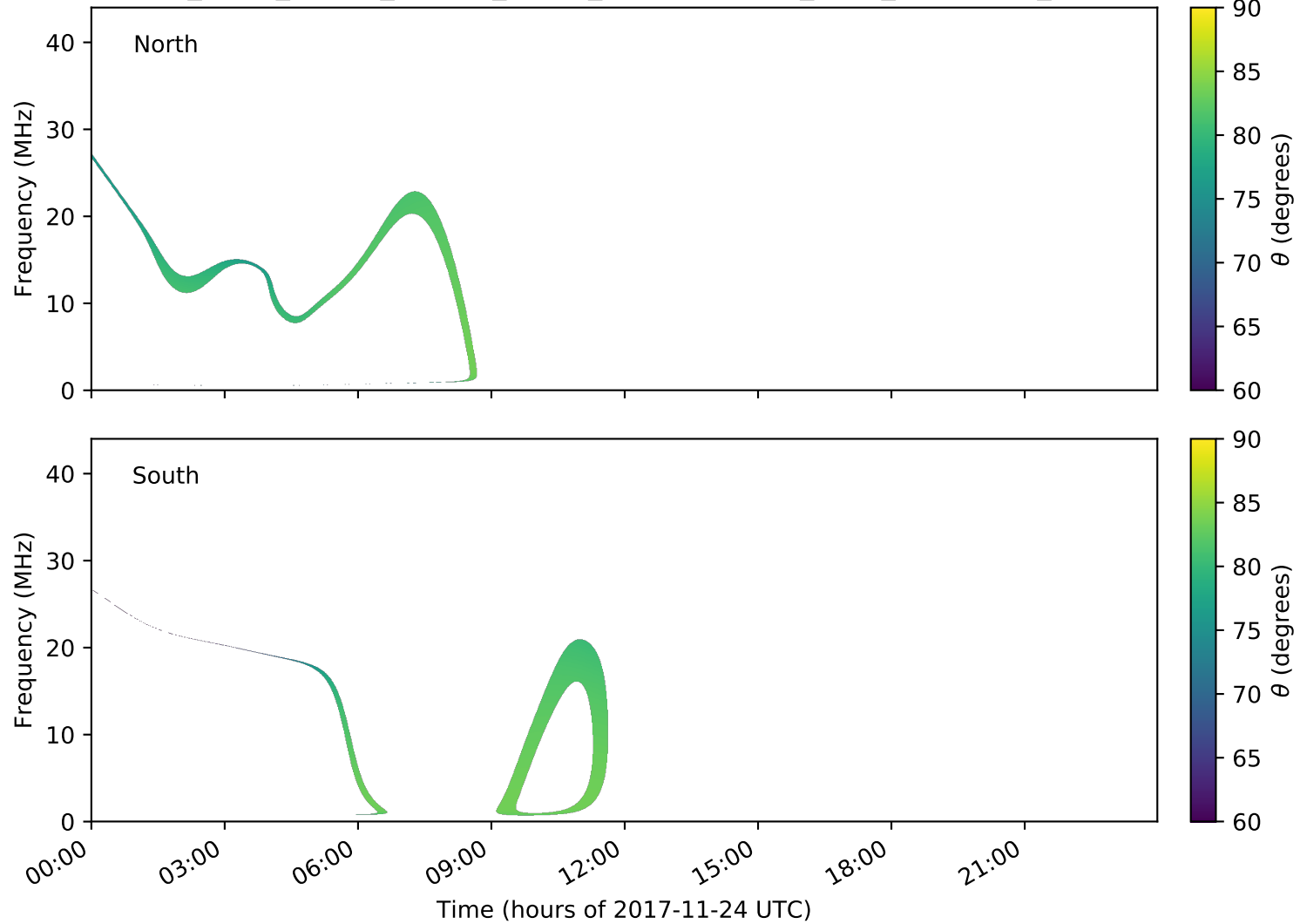
expres_earth_jupiter_europa_jrm09_lossc-wid1deg_3kev_20171124_v01.cdf
