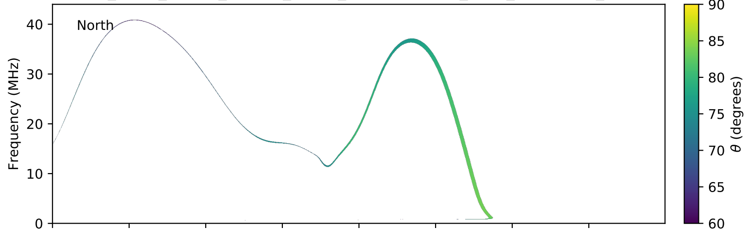
expres_earth_jupiter_europa_jrm09_lossc-wid1deg_3kev_20171120_v01.cdf
