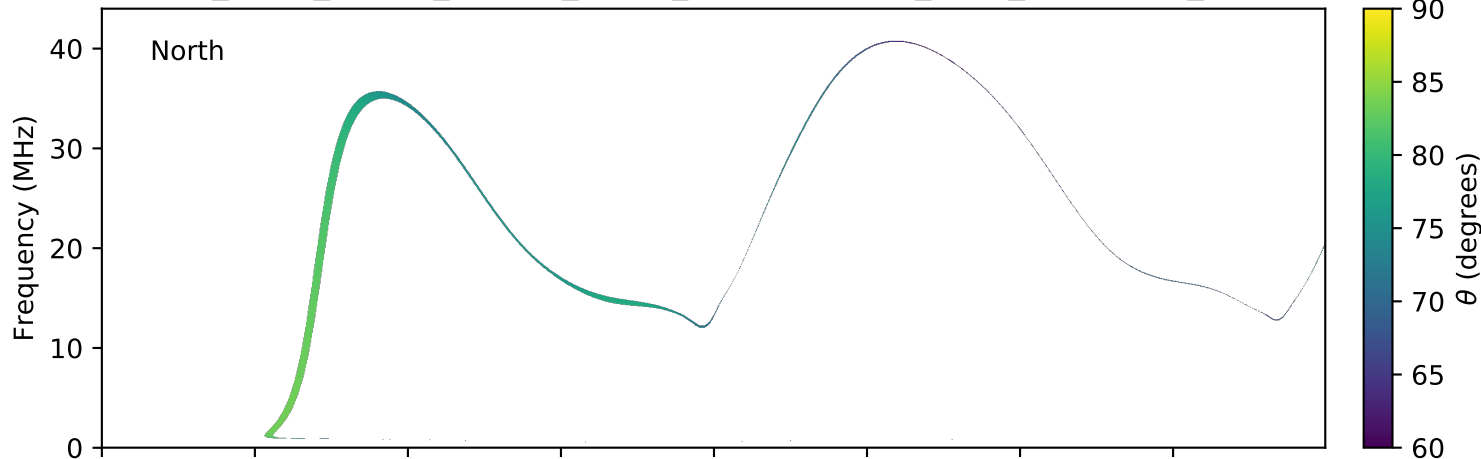
expres_earth_jupiter_europa_jrm09_lossc-wid1deg_3kev_20171112_v01.cdf
