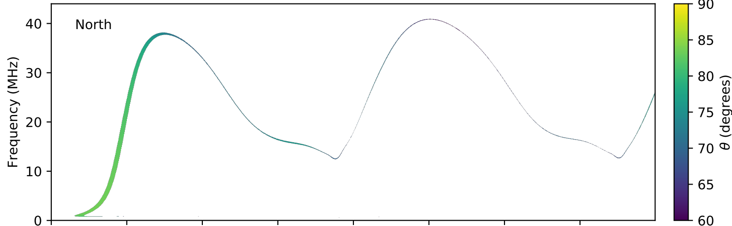
expres_earth_jupiter_europa_jrm09_lossc-wid1deg_3kev_20171105_v01.cdf
