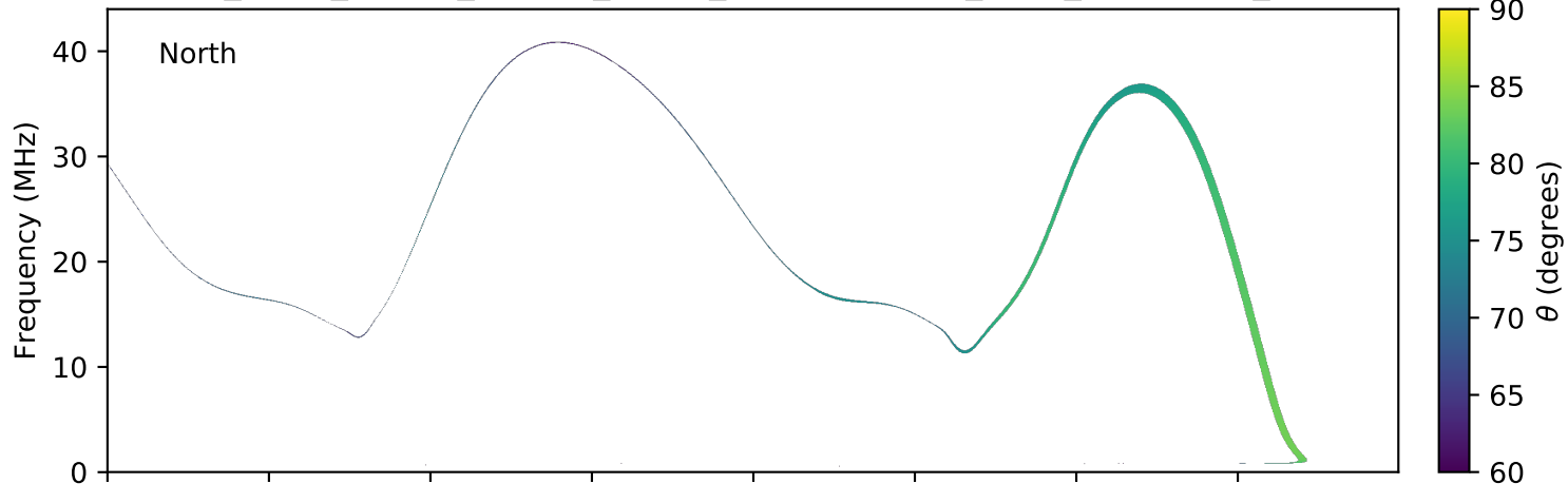
expres_earth_jupiter_europa_jrm09_lossc-wid1deg_3kev_20171102_v01.cdf
