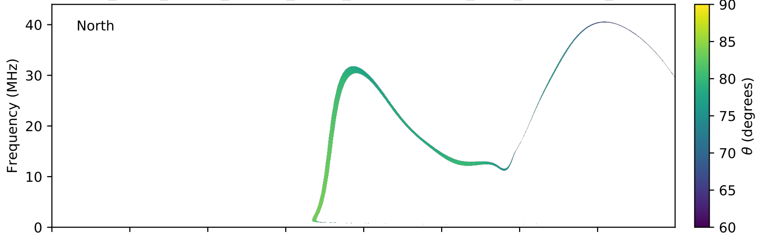
expres_earth_jupiter_europa_jrm09_lossc-wid1deg_3kev_20171101_v01.cdf
